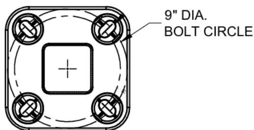
Figure 4.5. Anchor Base Detail
