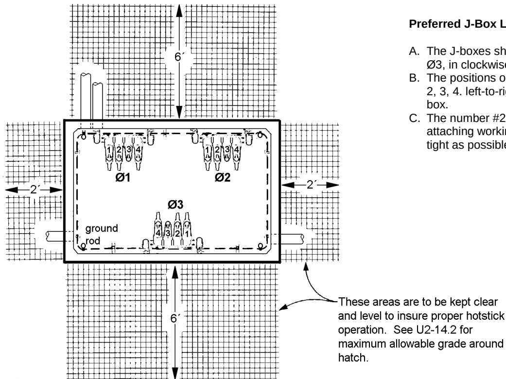
Figure 6. J-Box Locations and Operating Clearances
