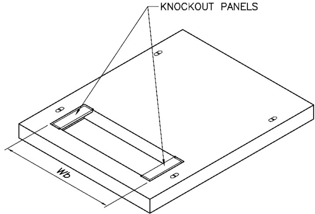
Figure 3.2b. Knockout Panel Detail, Stock No. 013724
