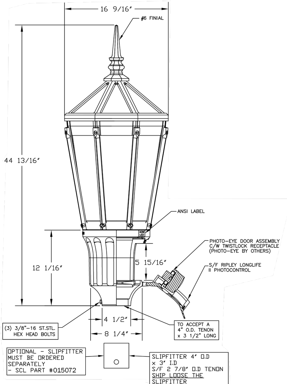
Figure 4.9. Luminaire Dimensions
