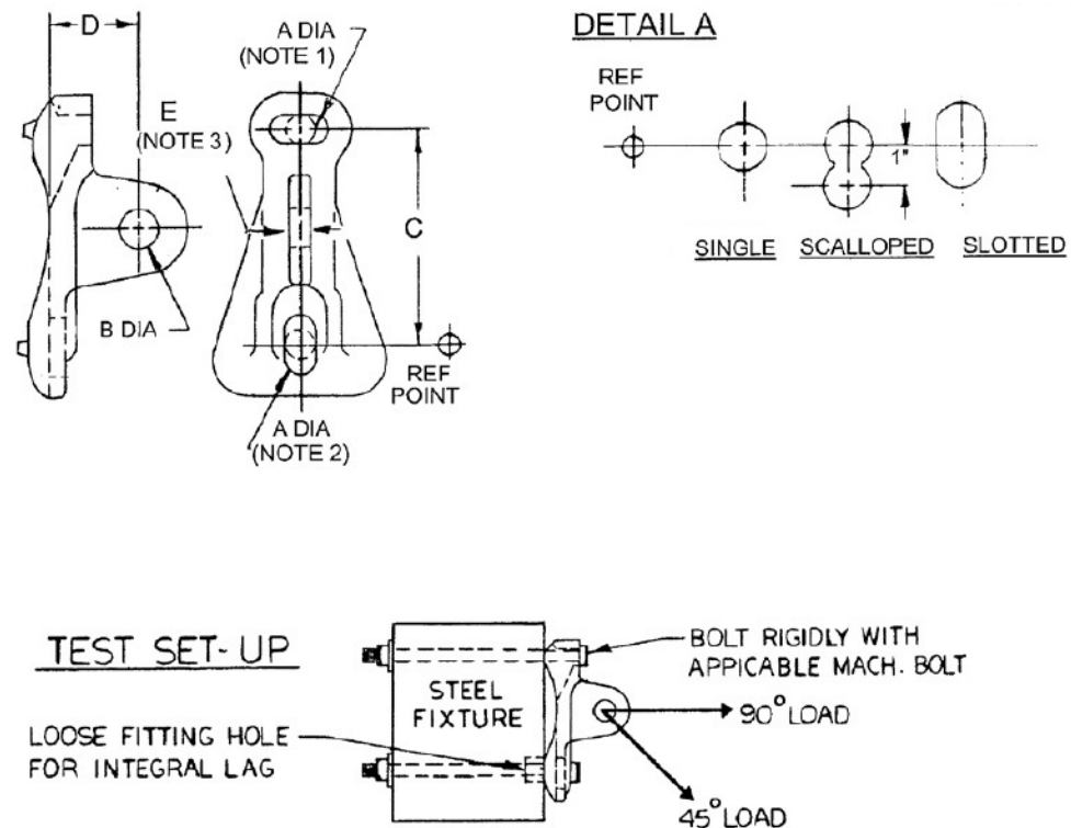
Figure 4. Pole Eye Plate Dimensions
