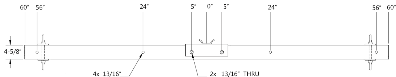
Figure 5.2c. Front View Dimensions
