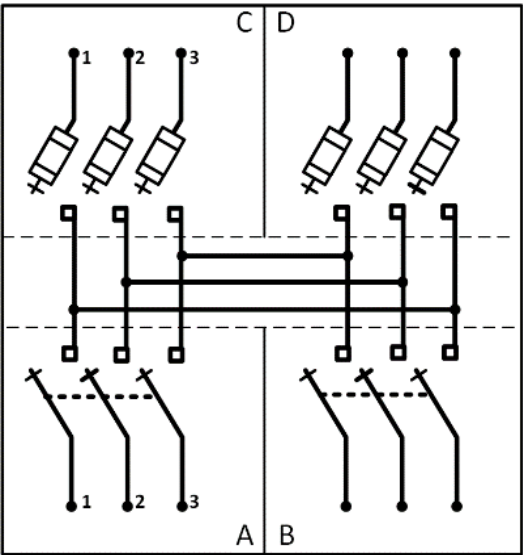
Figure 10.2. PMH-9 Switchgear Connection Diagram
