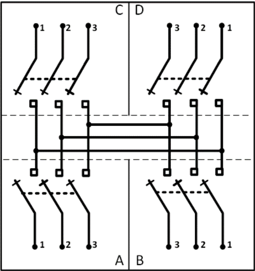
Figure 10.3. PMH-10 Switchgear Connection Diagram
