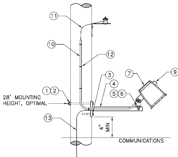
Figure 3.2. Single Floodlight Installation
