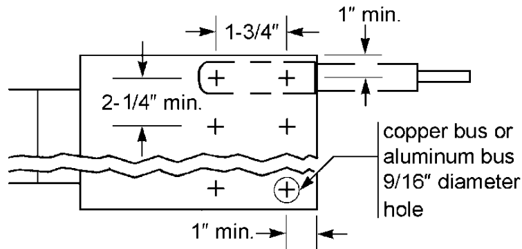
Figure 3g. Hole Spacing, Two-Hole Horizontal Connection
