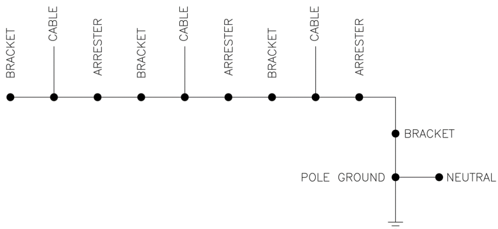
Figure 3.2c. Three-Phase 600 A Termination Grounding
