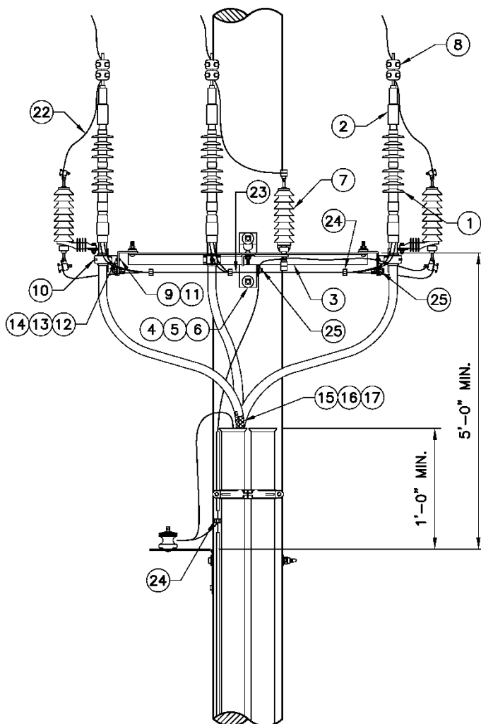
Figure 3.1b. Three-Phase 600 A Termination Assembly
