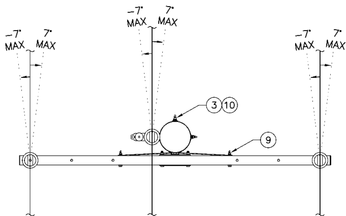
Figure 3a. Allowable Line Angle Range
