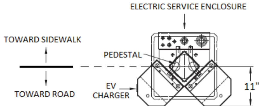
Figure 4.3c. Equipment Orientation
