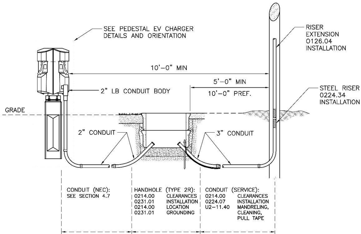
Figure 4.3a. Pedestal EV Charger Installation
